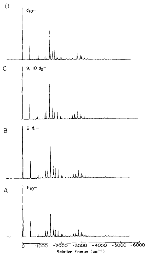
FIG. 2. 0^0 -level fluorescence spectra of the various anthracene species. The energy scale is relative to the h_{10}^0 band. Experimental conditions: laser-to-nozzle distance ( \equiv X ) = 5 mm, sample temperature ( \equiv T ) = 150 °C, pin-hole diameter ( \equiv D ) = 150 \mu m, carrier gas pressure ( \equiv P ) = 45 psi N_2 , excitation bandwidth ( \equiv BW ) = 2 Å, monochromator resolution ( \equiv R ) \approx 0.4 Å.
