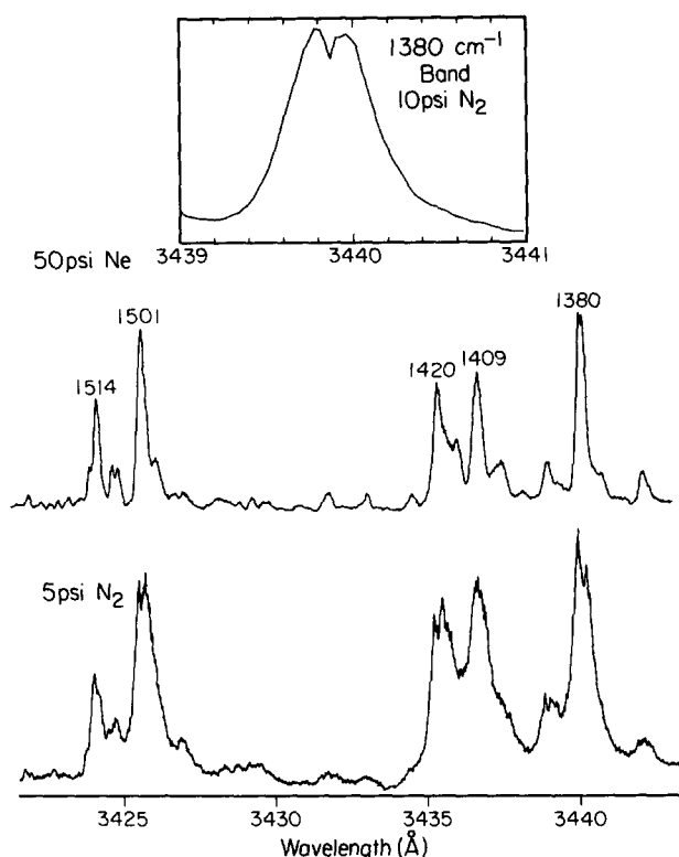
FIG. 23. Fluorescence excitation spectra of h_{10} -anthracene in the S_1 + 1350 to S_1 + 1550 \text{cm}^{-1} region for different carrier gas conditions. The spectra were taken with the pulsed nozzle system and are normalized. Prominent bands are labeled in the neon spectrum. Besides the general broadening of the spectrum, note the splitting of the 1380, 1420, and 1501 \text{cm}^{-1} bands when the carrier gas changes from 50 psi Ne to 5 psi \text{N}_2 . The splitting of the 1380 \text{cm}^{-1} band is apparent in the inset of the figure.
