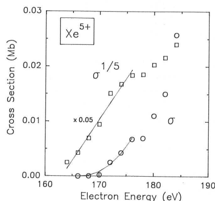
FIG. 13. Threshold cross sections for Xe^{5+} production. The fitting parameters for the power law expression to \sigma are E_0=166 and n=2.32 . The units for \sigma^{1/5} are Mb^{1/5} .
