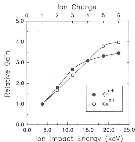
FIG. 5. MCP gain for Kr n + and Xe n + as a function of ion impact energy and corresponding ion charge.
