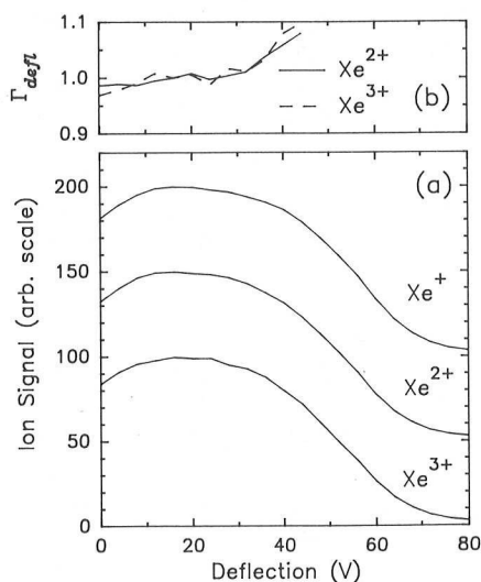
FIG. 4. (a) Measured deflection functions for Xe + , Xe 2+ , and Xe 3+ . (b) Intensity ratio f_{\text{defl}}^R / f_{\text{defl}}^M is for R = \text{Xe}^+ and M = \text{Xe}^{2+} and Xe 3+ .
