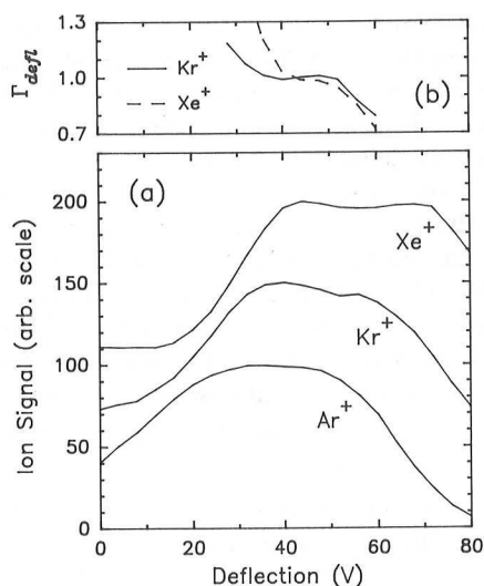
FIG. 3. (a) Measured deflection functions for Ar + , Kr + , and Xe + representing ion-signal strength vs deflection voltage. All curves are normalized to a 0–100 scale and offset by 50 units for clarity. (b) The intensity ratio f_{\text{defl}}^R / f_{\text{defl}}^M , where R = \text{Ar} and M = \text{Kr, Xe} , constitutes the correction factor \Gamma_{\text{defl}} in Eq. (2).
