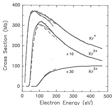
FIG. 7. Cross sections for \text{Kr}+e\rightarrow\text{Kr}^{n+}+(n+1)e for n=1-3 . . . ., present data; —, SHM data; — —, WBHF data.
