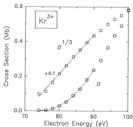
FIG. 12. Threshold cross sections for Kr^{3+} production. The fitting parameters for the power-law expression to \sigma are E_0=74 and n=2.14 . The units of \sigma^{1/3} are Mb^{1/3} .
