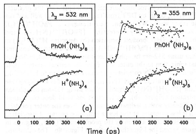
Figure 4. Time-resolved measurements of reactant [\text{PhOH}]^+(\text{NH}_3)_n ( R^+ ) and product \text{H}^+(\text{NH}_3)_n ( P^+ ) signals for cluster size n = 6 : (a) \lambda_2 = 532\text{-nm} , two-photon ionization and (b) \lambda_2 = 355\text{-nm} , one-photon ionization. We show \text{H}^+(\text{NH}_3)_4 traces for n = 4 and n = 5 because, typically, two and one solvent molecules evaporate at these respective ionization energies following DPT (ref 13b). The R^+ data were fitted to eq 1 for 1/k = 65 \text{ ps} , f_a = 0 , i_a/i_b = 2.0 , and f_b = 0.96 ( \lambda_2 = 532 \text{ nm} ) and 0.65 ( \lambda_2 = 355 \text{ nm} ). The P^+ data were fitted to a double exponential function (described in paper 1, ref 12) with time constants 65 and 350 ps.
