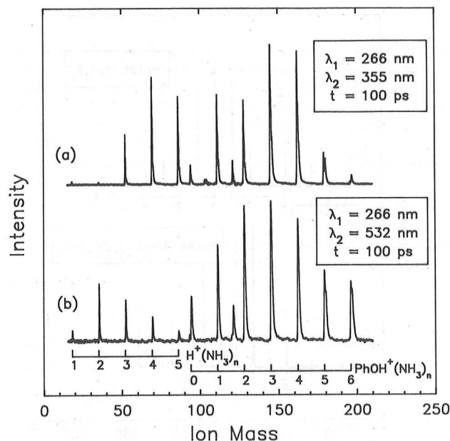
Figure 3. Two-color picosecond delayed ionization REMPI mass spectra for (a) \lambda_2 = 355\text{-nm} , one-photon ionization and (b) \lambda_2 = 532\text{-nm} , two-photon ionization. Excitation conditions were \lambda_1 = 266 \text{ nm} ( \sim 20 \mu\text{J} /pulse, 2-mm diameter), \lambda_2 = 355 \text{ nm} ( \sim 0.5 \text{ mJ} /pulse, 3-mm diameter), and \lambda_2 = 532 \text{ nm} ( \sim 1 \text{ mJ} /pulse, 3-mm diameter). Expansion conditions were 10% \text{NH}_3 in He at 35 psi and phenol at 60^\circ\text{C} . The signal at 121 amu is believed to be an impurity. Deflection plates were adjusted to emphasize lower masses.
