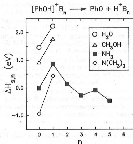
Figure 9. Enthalpies for stepwise solvation of DPT in [\text{PhOH}]^+\text{B}_n clusters. The first point for each solvent B corresponds to the bimolecular gas-phase reactants [\text{PhOH}]^+ + \text{B} .
