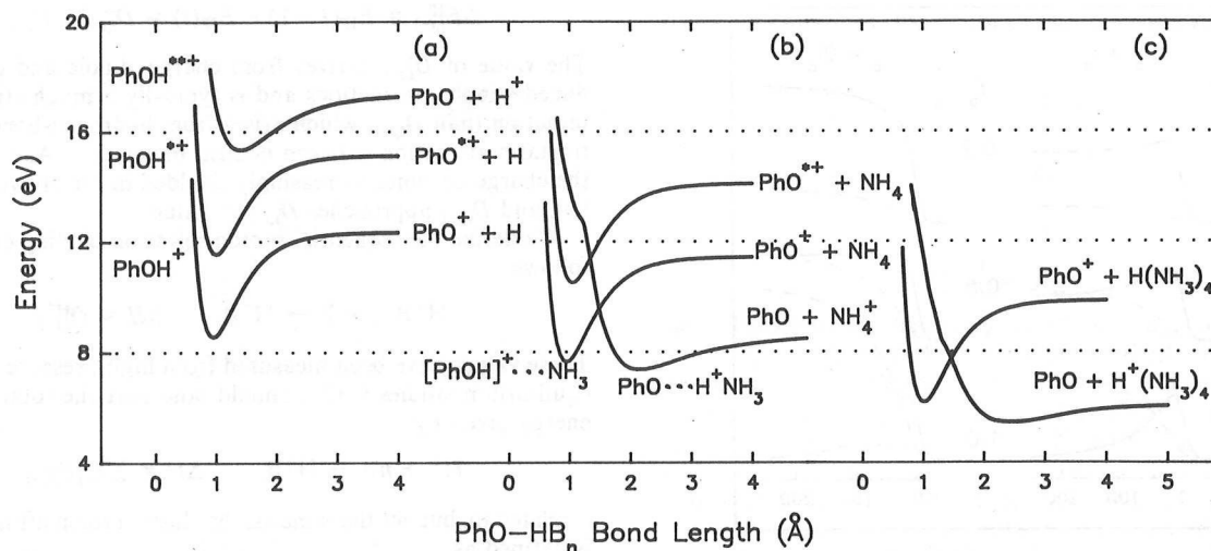
Figure 8. Approximate [\text{PhOH}]^+(\text{NH}_3)_n cluster ion potential energy curves for the reactive \text{PhOH} coordinate: (a) n = 0 , (b), n = 1 , and (c) n = 4 . Energies are relative to the unsolvated \text{PhOH}^+ cation.
