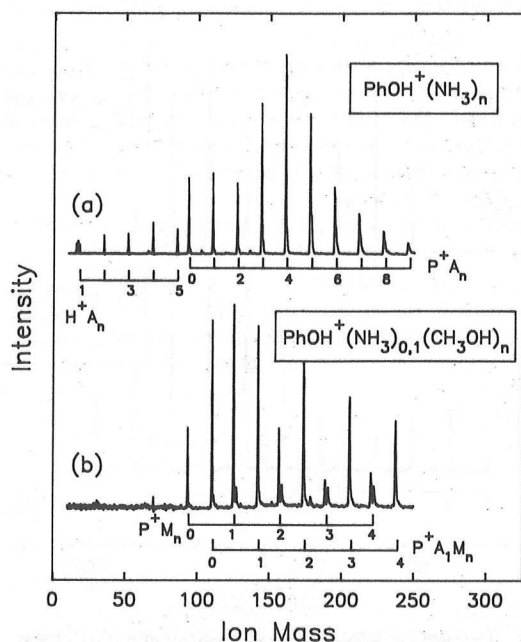
Figure 5. One-color nanosecond REMPI mass spectra at 280 nm: (a) pure (\text{NH}_3)_n solvation and (b) mixed solvation involving \text{NH}_3(\text{CH}_3\text{OH})_n . P = phenol, A = \text{NH}_3 , and M = \text{CH}_3\text{OH} . The peaks that appear at 2 amu above the \text{P}^+\text{A}_n series are presumed to be due to demethylation (loss of 15 amu) from \text{P}^+\text{A}_1\text{M}_n cluster ions.
