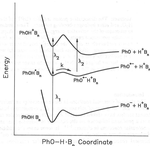
Figure 1. Energy diagram for \text{PhOH}(\text{NH}_3)_n consistent with a cluster size of n \sim 5 . Excitation scheme showing how delayed ionization by \lambda_2 can produce cluster ions in the outer potential well for reactive \text{PhOH}^+\text{B}_n clusters excited by \lambda_1 . The \lambda_2 ionization may occur by more than one photon. Pictorial electronic structures are given for the inner well, transition-state, and outer well complexes.
