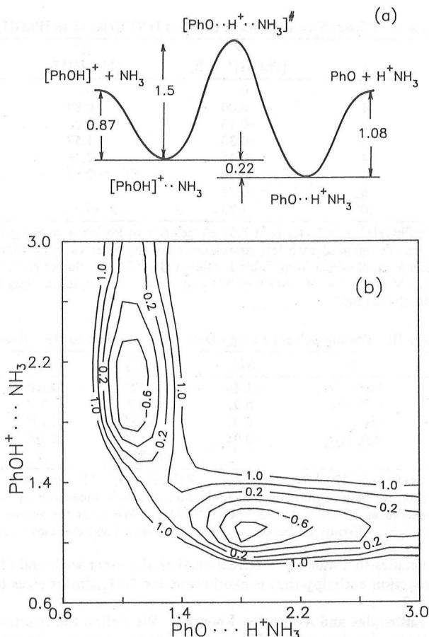
Figure 10. Reactive potential energy surface for [\text{PhOH}]^+ + \text{NH}_3 : (a) minimum-energy reaction coordinate and (b) 2D collinear potential energy surface. Energies (eV) are relative to reactant asymptotic limit. Contour spacings are 0.4 eV.
