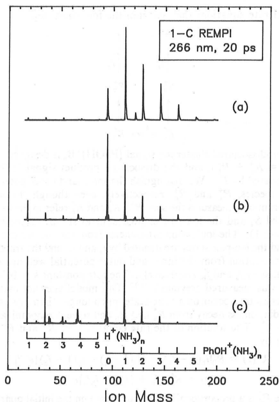
Figure 2. One-color picosecond REMPI mass spectra with 20-ps 266-nm radiation of varying pulse intensity: (a) two-photon signals ( \sim 20 \mu\text{J} /pulse, 2-mm diameter), (b) appearance of \text{H}^+(\text{NH}_3)_n at the three-photon level ( \sim 80 \mu\text{J} /pulse, 2-mm diameter), (c) appearance of aromatic fragments at the four-plus photon level ( \sim 80 \mu\text{J} /pulse, \sim 300\text{-}\mu\text{m} diameter). Deflector voltage was adjusted to emphasize lower masses.
