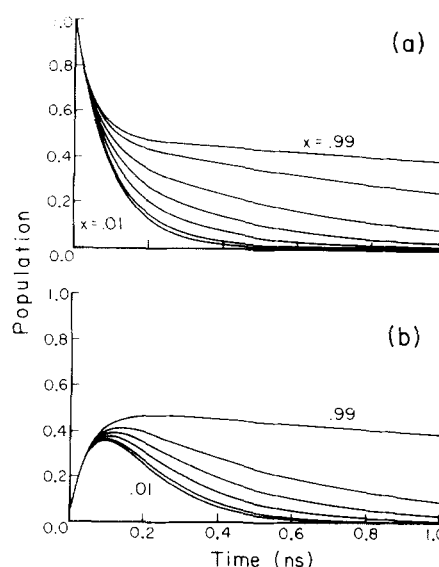
FIG. 6 Calculated time dependence of (a) \{|I\rangle\} and (b) \{|p\rangle\} for A_p \approx A_I . Input parameters for A_I were k_{lp} = 1 \times 10^{10} \text{ s}^{-1} and k_{lg} = k_{lg}^r = 4 \times 10^8 \text{ s}^{-1} . Parameters for A_p were k_{pl} = xA_p where A_p = k_{pl} + k_{pg} = 1 \times 10^{10} \text{ s}^{-1} . Calculated curves are for values x = 0.99, 0.90, 0.70, 0.50, 0.30, 0.10, 0.01 , from top to bottom.
