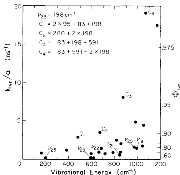
FIG. 8. Rate and quantum yield of IVR as a function of S_1 vibrational energy. The rate is expressed as a function of \alpha which includes the radiative rate constants from the |s\rangle and \{|l\rangle\} states as well as any systematic errors involved in distinguishing between relaxed and unrelaxed fluorescence in SVL dispersed fluorescence spectra.
