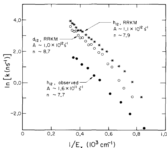
FIG. 15. Effective temperature analysis of reaction rates as a function of E_x . The data were analyzed according to Eq. (17) using a barrier of E_0 = 1150 cm -1 . The symbols used to denote the RRKM data correspond to the set of data plotted in Fig. 16.
