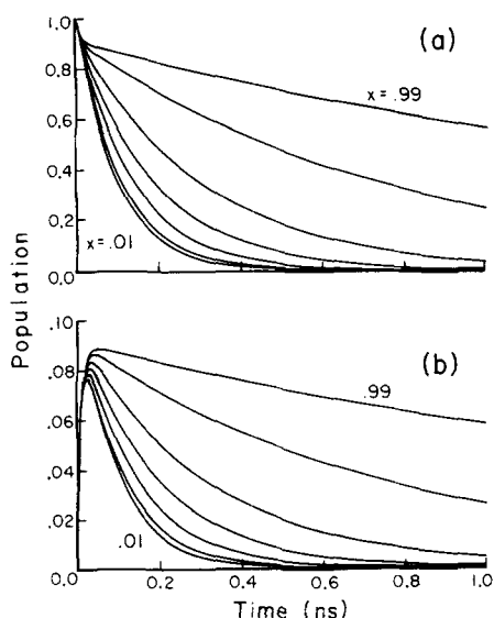
FIG. 7. Calculated time dependence of (a) \{|I\rangle\} and (b) \{|p\rangle\} for \Lambda_p \approx 10A_l . Input parameters are the same as in Fig. 7 except that \Lambda_p = 1 \times 10^{11} \text{ s}^{-1} . Note the change of population scale for (b).
