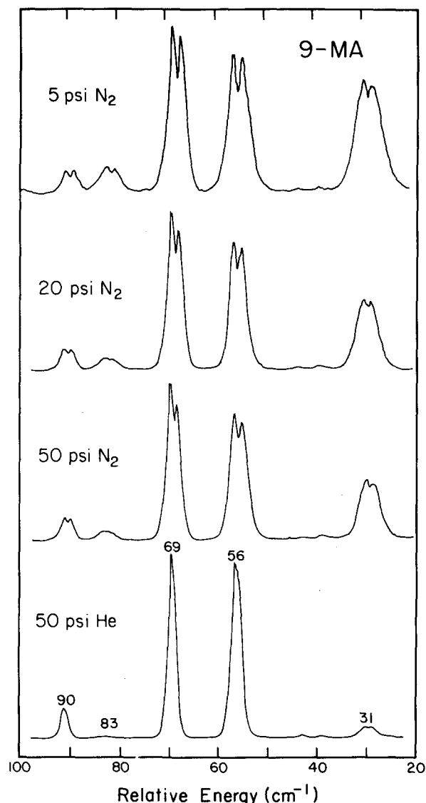
FIG. 8. High resolution spectra of the low frequency region of 9-methylantracene as a function of carrier gas and backing pressure illustrating the variation of the torsional (hot) band intensity and band shape. Note rotational band splitting. This latter feature was observed and analyzed for anthracene in Ref. 6.
