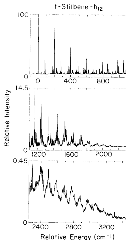
FIG. 4. Fluorescence excitation spectra of t -stilbene- h_{12} for the ^1B_u \leftarrow ^1A_g electronic transition. Spectra were recorded under expansion conditions of 50 psi He and 80 °C sample temperature. All other conditions are given in the experimental.
