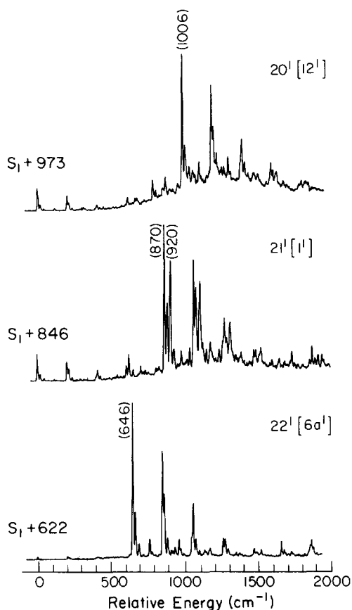
FIG. 3. Dispersed fluorescence spectra of t -stilbene- h_{12} following SVL excitation to benzene type modes in S_1 . The false origins represent the A_1^+ emission following A_0^+ excitation. Hence, the value of the frequency displaced from the excitation frequency (denoted in parentheses) represents an interval in S_0 .
