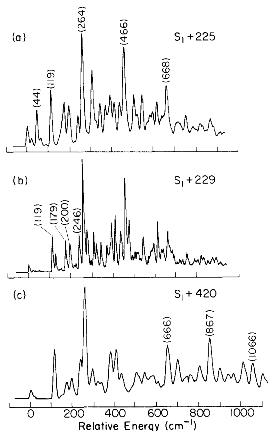
FIG. 10. Dispersed fluorescence spectra from S_1 levels at (a) 225 \text{ cm}^{-1} ; (b) 229 \text{ cm}^{-1} ; and (c) 420 \text{ cm}^{-1} . The similarity of the S_1 + 225 and 229 \text{ cm}^{-1} spectra is indicative of Fermi resonance. A frequency perturbation is apparent in that the S_1 + 420 \text{ cm}^{-1} spectrum, which is assigned to the 225 + 198 \text{ cm}^{-1} combination, does not appear at the sum frequency.
