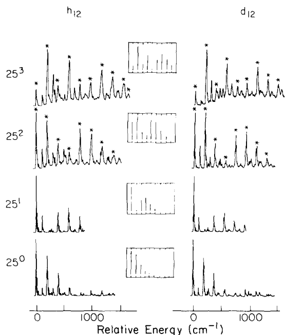
FIG. 7. SVL dispersed fluorescence spectra following excitation into the fundamental and overtones of the \nu_{25} symmetric C_e C_e \phi in plane bend mode. The intensity distribution of the 25_n^m progressions were calculated for a series of geometry changes in t -stilbene using Franck-Condon analysis. The best fit to all spectra was obtained for a distortion parameter \gamma along the \nu_{25} normal coordinate of 0.94. The calculated results for t -stilbene- h_{12} are illustrated in the inserts.
