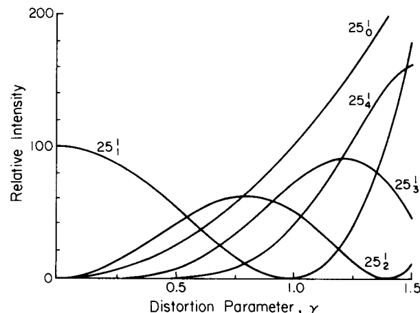
FIG. 15. Calculated Franck-Condon fluorescence intensity distribution for the 25_n^o progression. The parameter \gamma denotes the change in the \nu_{25} normal coordinate that occurs upon ^1B_g \leftrightarrow ^1A_g electronic transition. The calculation applies to t -stilbene- h_{12} using the ground and excited state frequencies \nu_{25}'' = 204 \text{ cm}^{-1} and \nu_{25}' = 198 \text{ cm}^{-1} . Essentially identical results were obtained using the frequencies for the -d_{12} isomer.
