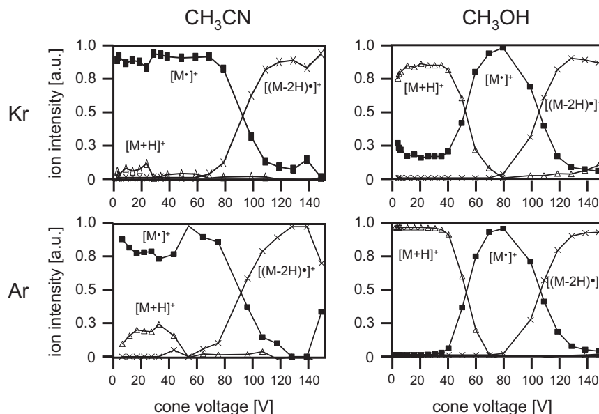
Figure 6. Plot of fractional signals for [M+H]^+ , [M]^+ and [(M-2H)]^+ for benzo[a]pyrene versus cone voltage in 100 \mu\text{L}/\text{min} flow of acetonitrile (left column) or methanol (right column) using a Kr lamp (top row) or an Ar lamp (bottom row). [M]^+ and [M+H]^+ have been corrected for isotopic abundances.
